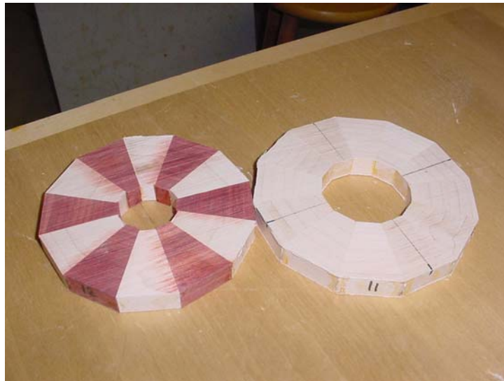
Figure 3 Alignment marks.
